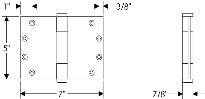
HMGWT5x7 Concealed Bearing Hinge 5" x 7"
