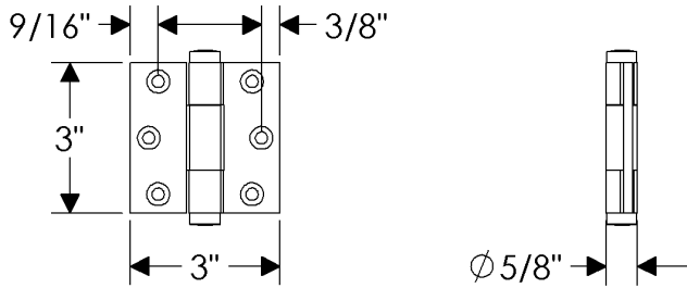
HNG3A Concealed Bearing Hinge 3" x 3"
