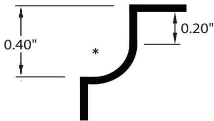
Cove
