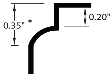
Roundover
